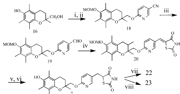
Scheme 2. Reagents: (i) NaH, MOMCl, DMF; (ii) 11, NaH, THF; (iii) Raney Ni, HCOOH; (iv) TZD, Piperidinium acetate, toluene; (v) 10% Pd/C, dioxane; (vi) gl. acetic acid, 10% H 2 SO 4 ; (vii) MCPBA; (viii) HCl.
